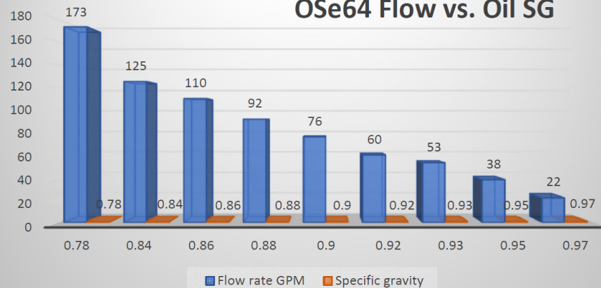
OSe64 Flow vs. Oil SG
