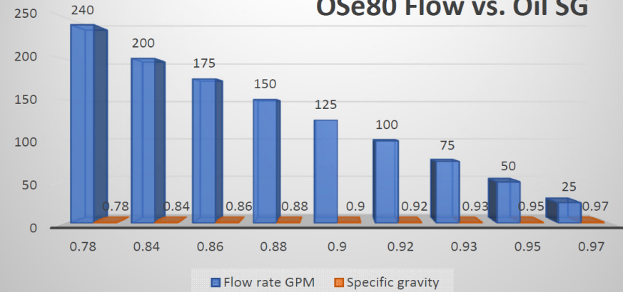
OSe80 Flow vs. Oil SG
