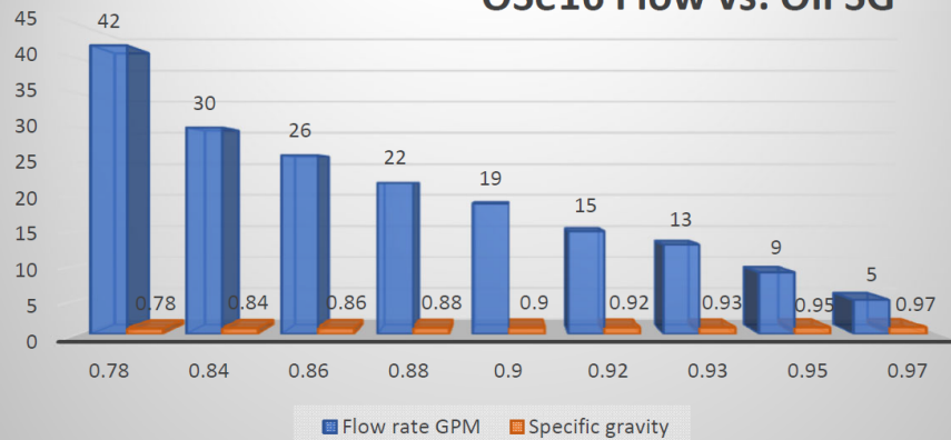
OSe16 Flow vs. Oil SG
