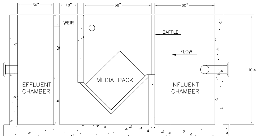
SECTIONAL SIDE VIEW
